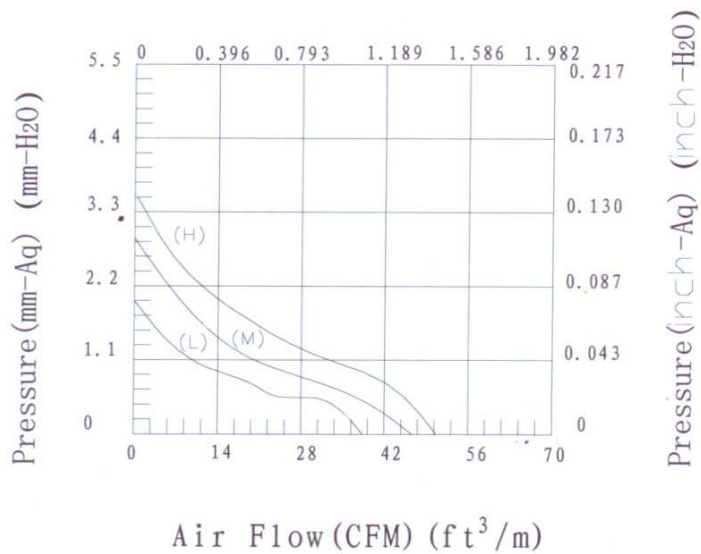
SPEEDY FAN PERFORMANCE CURVES Air Flow (CMM) ( M^3/m )
